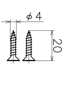
Installation Screw
